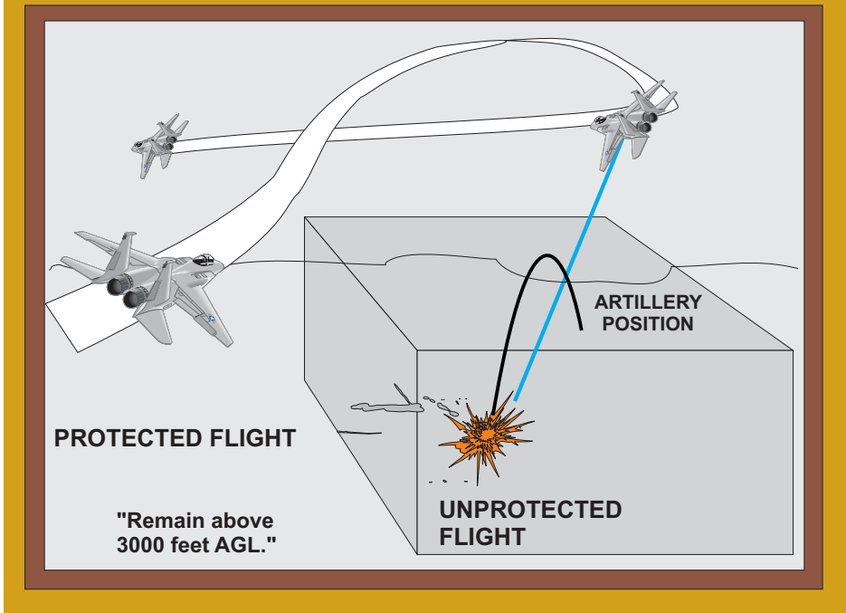
Figure V-4. Artillery-Close Air Support Aircraft Altitude Separation
